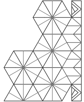
CORNER ELEVATION
