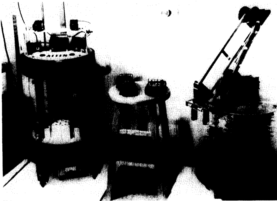
Fig. 1. The four MIT AI laboratory Mobots. Left-most is the first built Allen, which relies on an offboard LISP machine for computation support. The right-most one is Herbert, shown with a 24 node CMOS parallel processor surrounding its girth. New sensors and fast early vision processors are still to be built and installed. In the middle are Tom and Jerry, based on a commercial toy chassis, with single PALs (Programmable Array of Logic) as their controllers.
